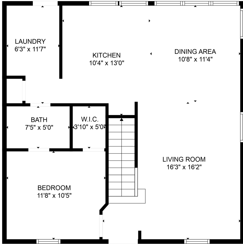
FLOOR 1
